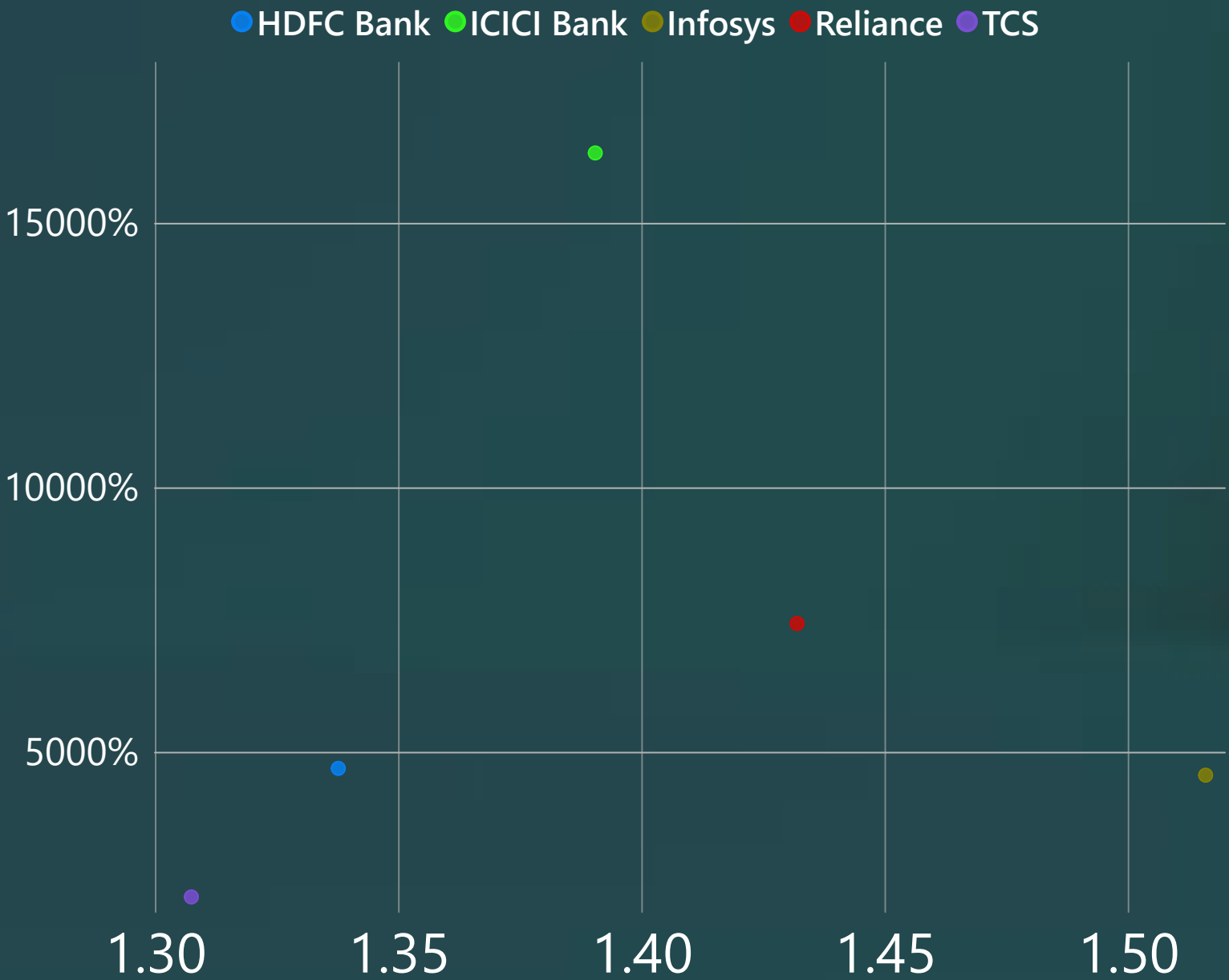
Volatility % and Total Return % by Company
